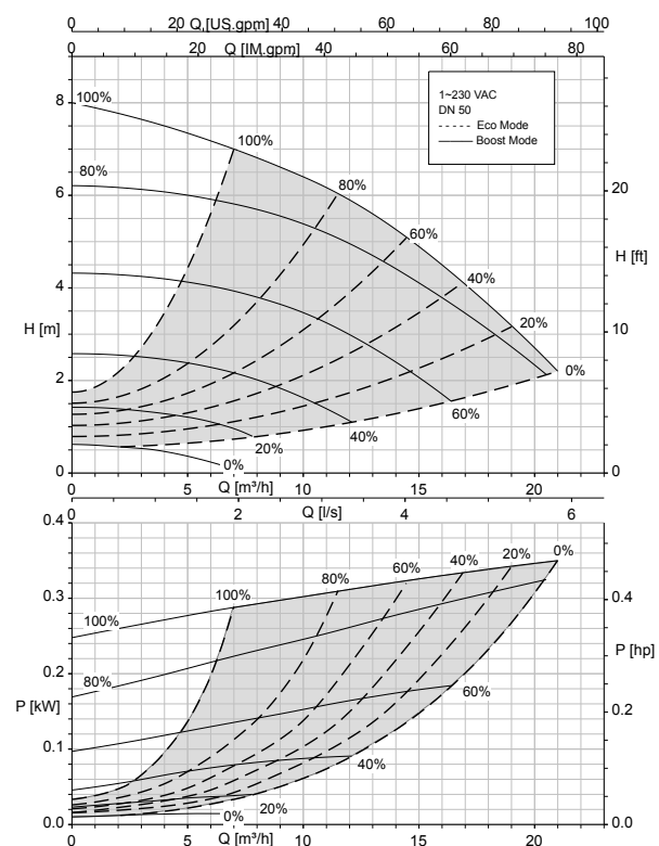
Calio 50-80 Boost-Mode, Eco-Mode
