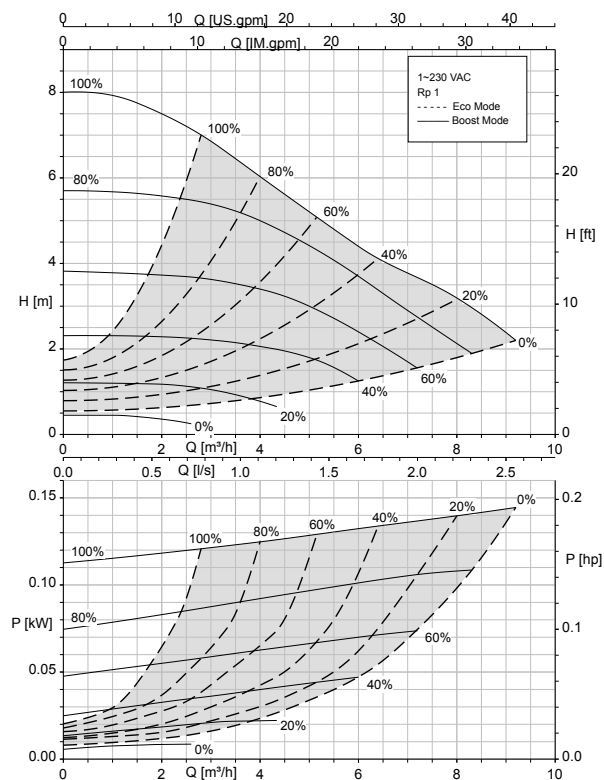
Calio 25-100 Boost-Mode, Eco-Mode
