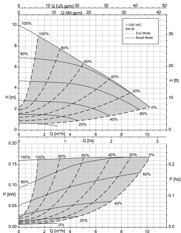
Calio 50-100 Boost-Mode, Eco-Mode
