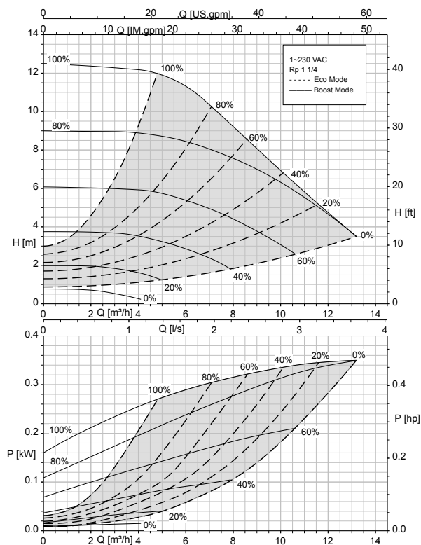
Calio 32-120 Boost-Mode, Eco-Mode
