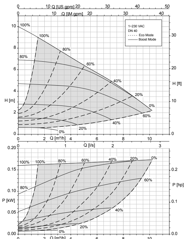
Calio 40-90 Boost-Mode, Eco-Mode
